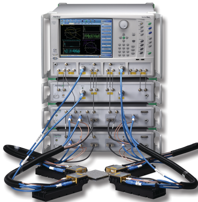
ME7838A4X 4-Port VNA
